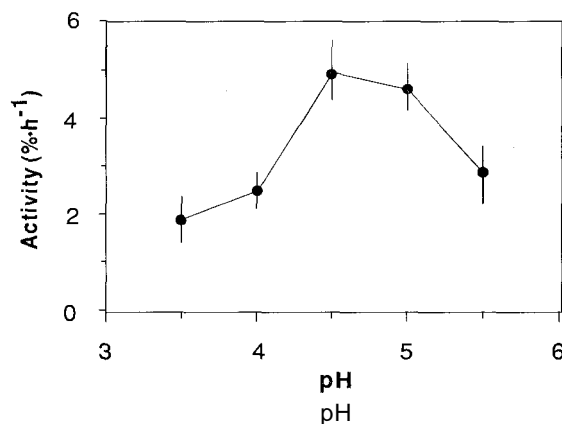
Fig. 7. pH dependence of the extension activity reconstituted by oat wall proteins. Heat-inactivated walls from cucumber hypocotyls were clamped in an extensometer as in Fig. 1 and placed in 50 mM sodium acetate buffers at pH 3.5, 4.0, 4.5, 5.0 or 5.5. After 20 min, the solutions were replaced with 0.4 mL of the corresponding buffer containing 10 μg oat-coleoptile wall proteins partially purified by DEAE-chromatography. The extension activity was calculated by subtracting the baseline rate without proteins from the linear rate (5-30 min) after the addition of the proteins, and expressed as % increase in length per h above the baseline rate. The data represent the means + SE ( n=5 to 8). The average baseline rate prior to addition of protein ranged between 2.52 and 2.96 (mm·min -1 or 3.0-3.55% per h) for all pH groups
